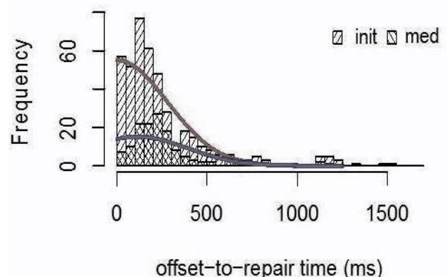
Figure 2: Histograms and fitted truncated gaussian distributions of offset-to-repair times, for initial and medial consonants (see text).
